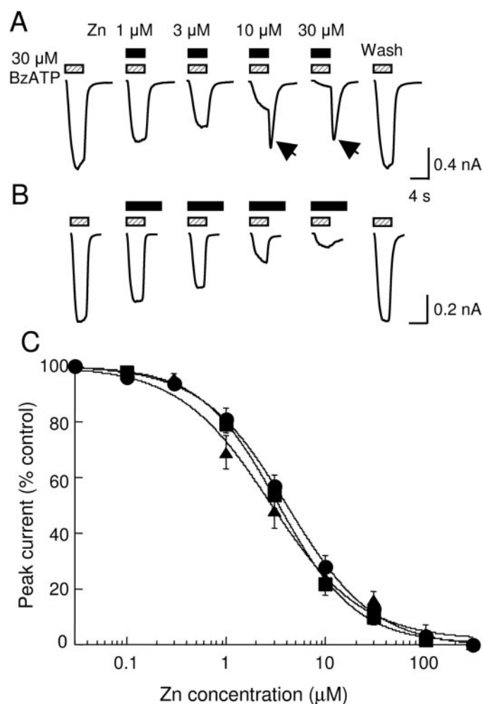
Fig. 1. Inhibition of P2X 7 receptor currents by zinc and rebound currents. A and B, representative BzATP-evoked currents in the presence of increasing concentrations of zinc. Note that there were robust rebound currents accompanying simultaneous washout of zinc and BzATP, as indicated by the arrows (the first protocol, A), which were absent in washout of BzATP in the persistent presence of zinc (the second protocol, B). C, zinc concentration-current response curves from all protocols as shown in A and B and described in text ( n = 3-8 for each point). ●, data from the first protocol ( IC_{50} = 4.6 \pm 0.9 \mu\text{M} , n = 8 ); ■, data from the second protocol ( IC_{50} = 5.9 \pm 1.2 \mu\text{M} , n = 4 ); ▲, data from preapplication of zinc ( IC_{50} = 5.6 \pm 1.4 \mu\text{M} , n = 4 ). These values were not significantly different from each other.
