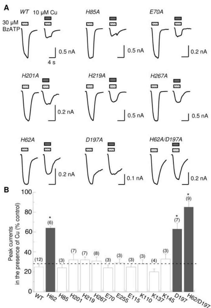
Fig. 4. Mutational effects on inhibition of BzATP-evoked P2X 7 receptor currents by copper. A, representative BzATP-evoked currents in the absence or presence of 10 μM copper at wild-type (WT) and indicated mutant P2X 7 receptors. B, summary of the results for all experiments as illustrated in A. The number of cells examined in each receptor is indicated in brackets. Significant attenuation in copper inhibition was seen at [D197A], [H62A] and [H62A/D197A] mutant receptors. *, p < 0.01 , compared with WT.
